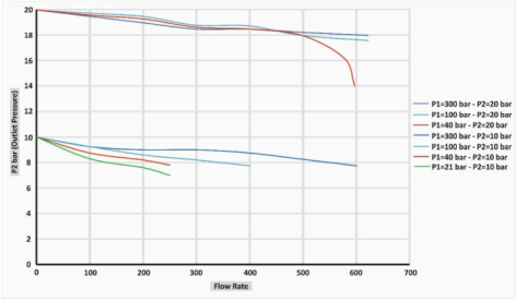
Flow Characteristics
